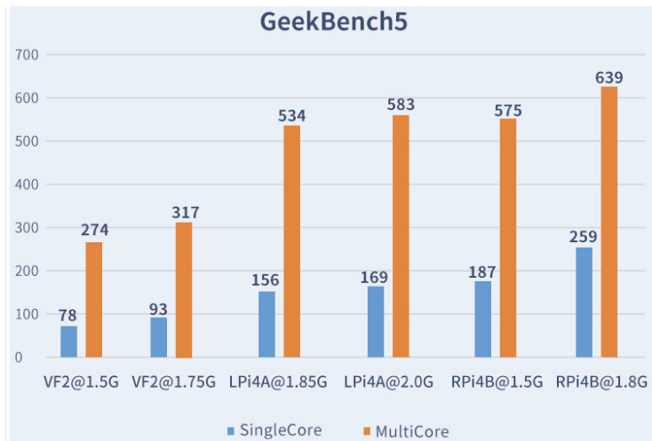
Figure 11: Various SBCs performance while running GeekBench5 (Integer and Floating-Point Workloads tests)
