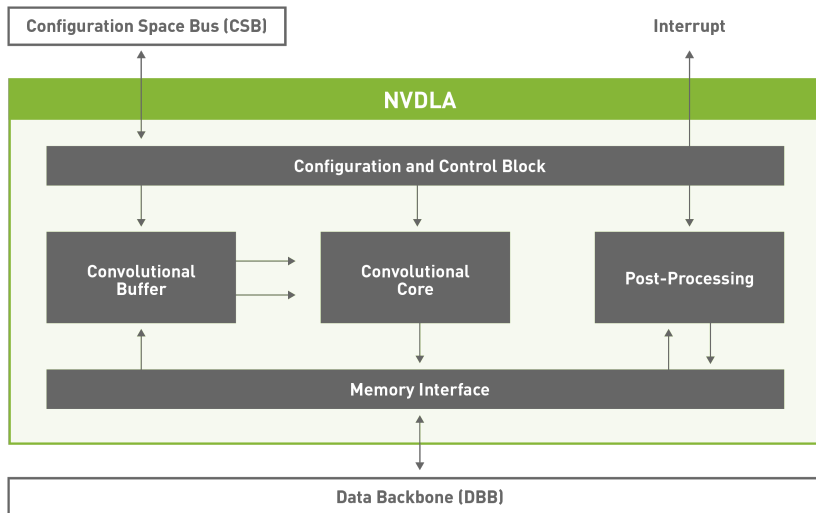
Figure 4: NVDLA Deep Learning MicroArchitecture
