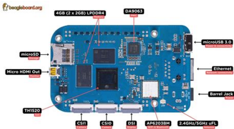
Figure 8: BeagleV-Ahead
